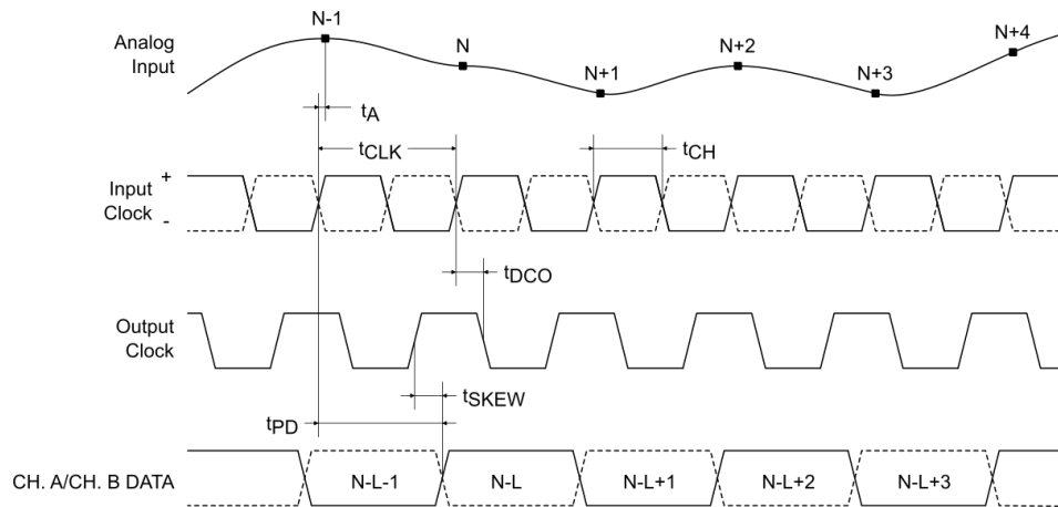
Figure 4: Parallel CMOS Output Mode Timing.
