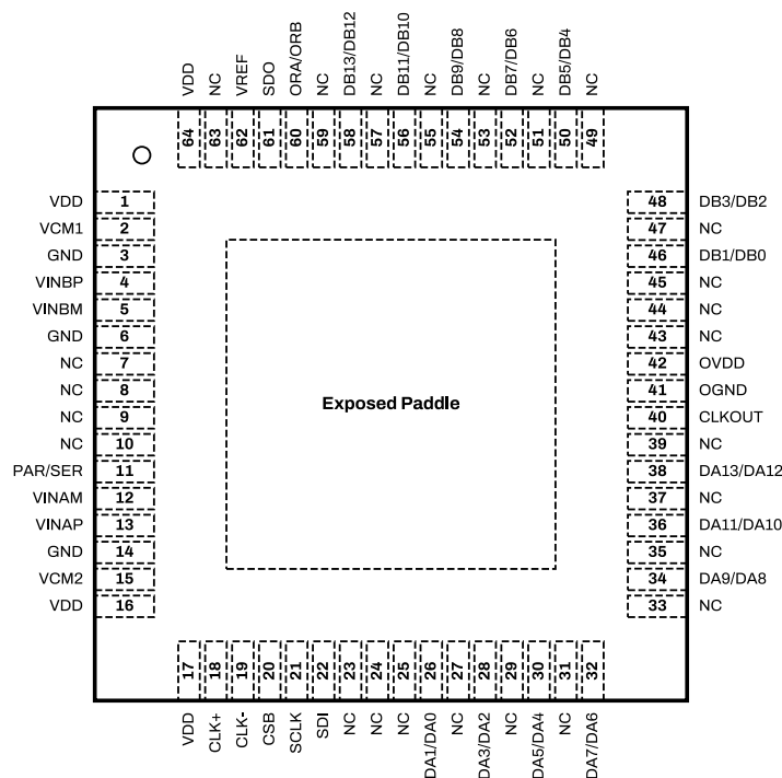
Figure 6: SD2140 Package Top View for Channel Multiplexed CMOS Configuration.
