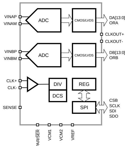
Figure 1: SD2140 Functional Block Diagram.
