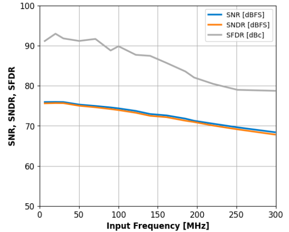
Figure 17: Single-Tone SNR, SNDR and SFDR vs. Input Frequency with f_S=25\text{MHz} .
