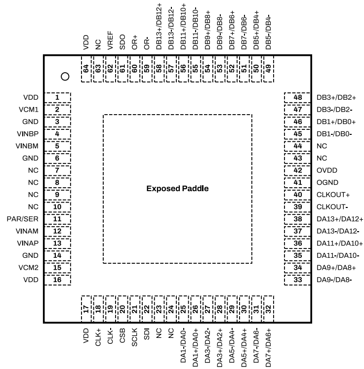
Figure 7: SD2140 Package Top View for Channel Multiplexed LVDS Configuration.
