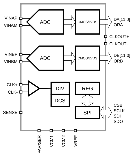
Figure 1: SD2142ET Functional Block Diagram.
