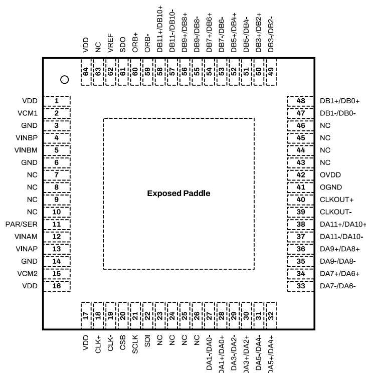
Figure 7: SD2142ET Package Top View for Channel Multiplexed LVDS Configuration.
