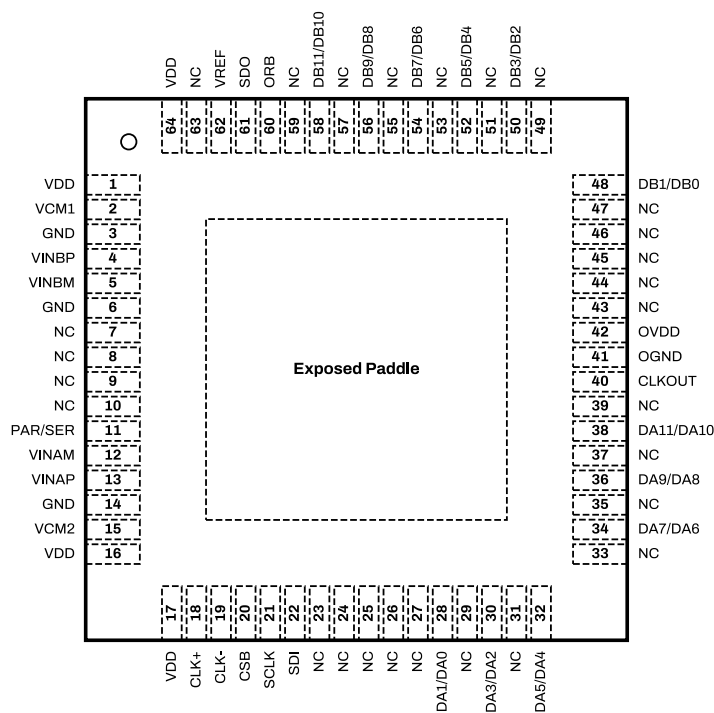
Figure 6: SD2142ET Package Top View for Channel Multiplexed CMOS Configuration.
