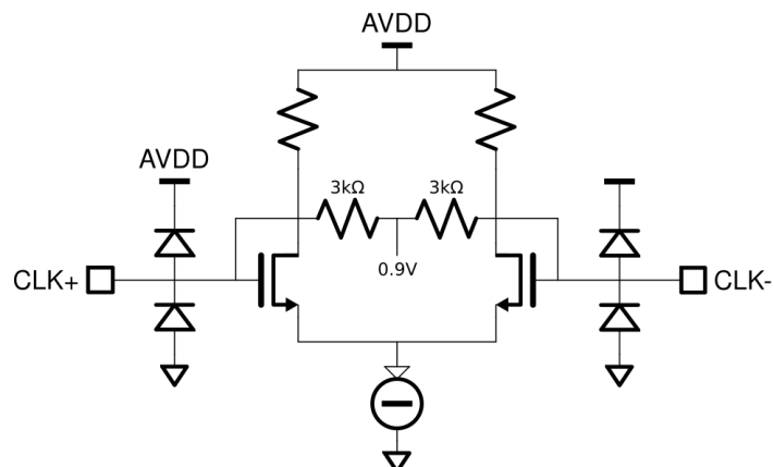
Figure 20: Equivalent Clock Input Circuit.
