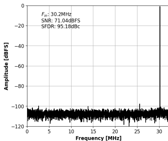
Figure 9: Single-Tone FFT with f_{IN}=30.2\text{MHz} .
