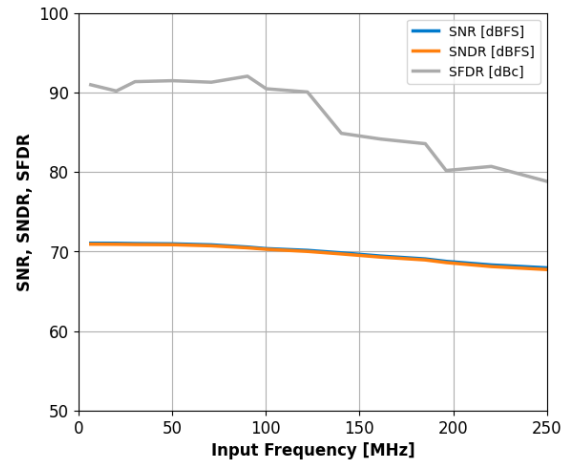
Figure 17: Single-Tone SNR, SNDR and SFDR vs. Input Frequency with f_S=65\text{MHz} .
