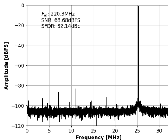
Figure 11: Single-Tone FFT with f_{IN}=220\text{MHz} .
