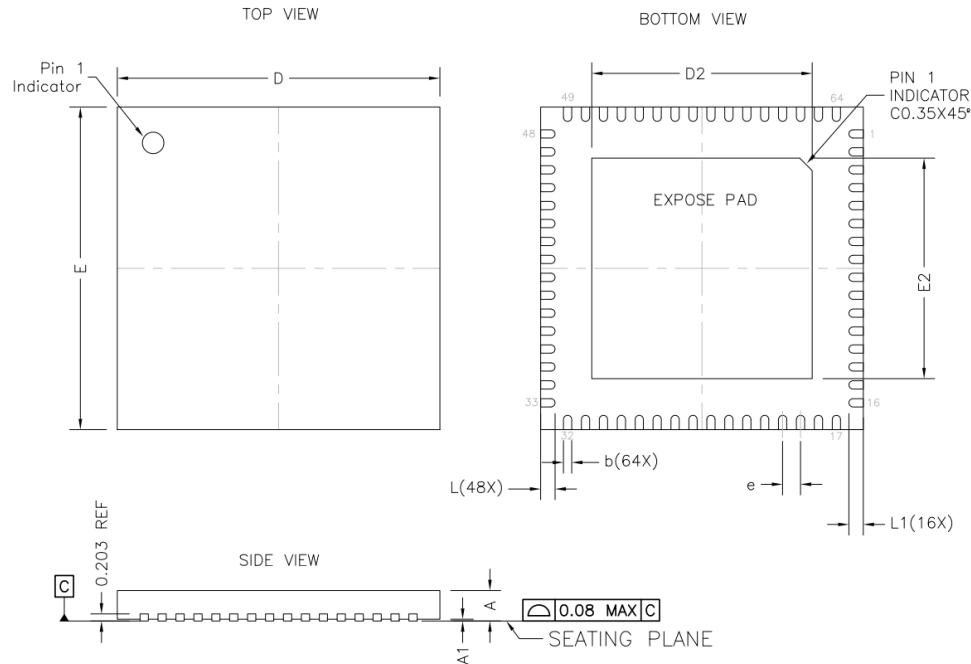
Figure 28: Package Dimensions.
