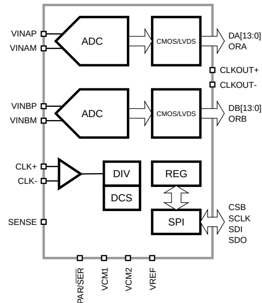
Figure 1: SD2142 Functional Block Diagram.
