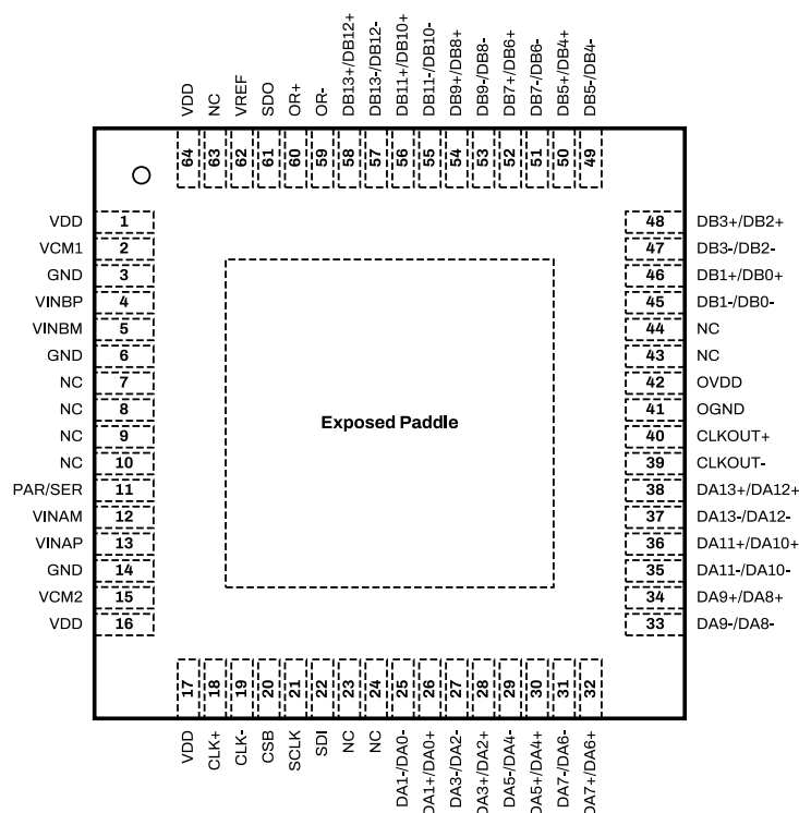
Figure 7: SD2142 Package Top View for Channel Multiplexed LVDS Configuration.
