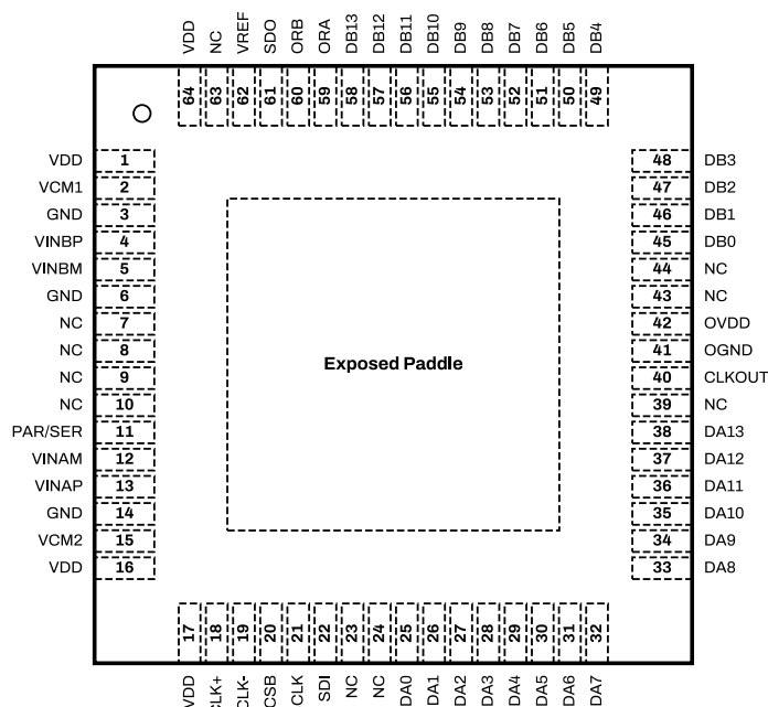
Figure 5: SD2142 Package Top View for Parallel CMOS Configuration.
