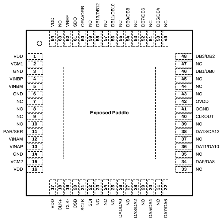
Figure 6: SD2142 Package Top View for Channel Multiplexed CMOS Configuration.
