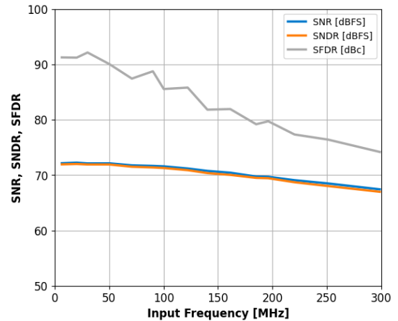
Figure 17: Single-Tone SNR, SNDR and SFDR vs. Input Frequency with f_S=80\text{MHz} .
