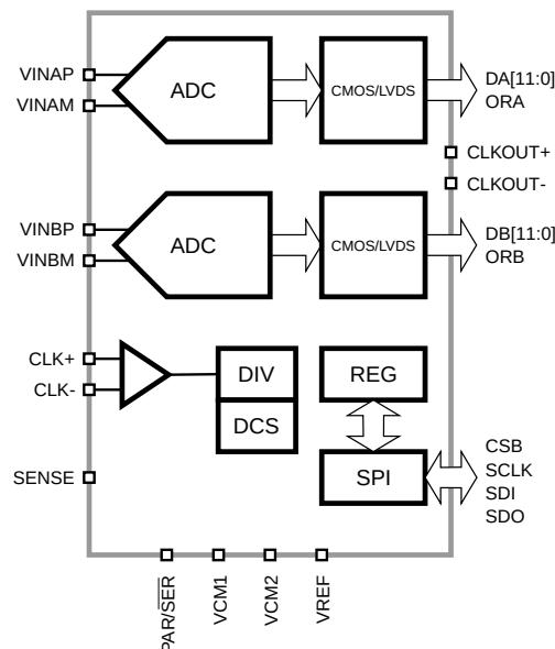
Figure 1: SD2143 Functional Block Diagram.
