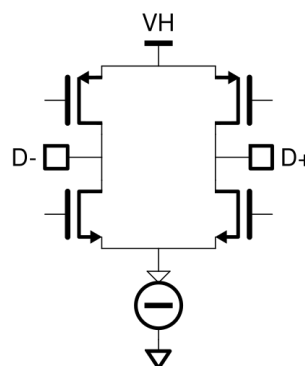
Figure 25: Equivalent LVDS output Circuit.
