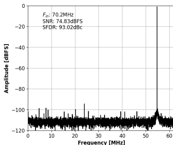
Figure 9: Single-Tone FFT with f_{IN}=70.2\text{MHz} .
