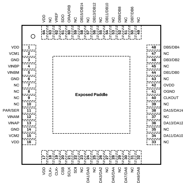
Figure 6: SD2180 Package Top View for Channel Multiplexed CMOS Configuration.
