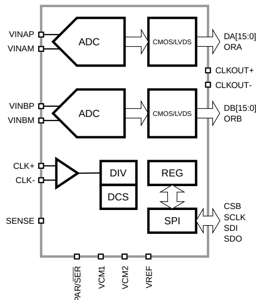
Figure 1: SD2180 Functional Block Diagram.
