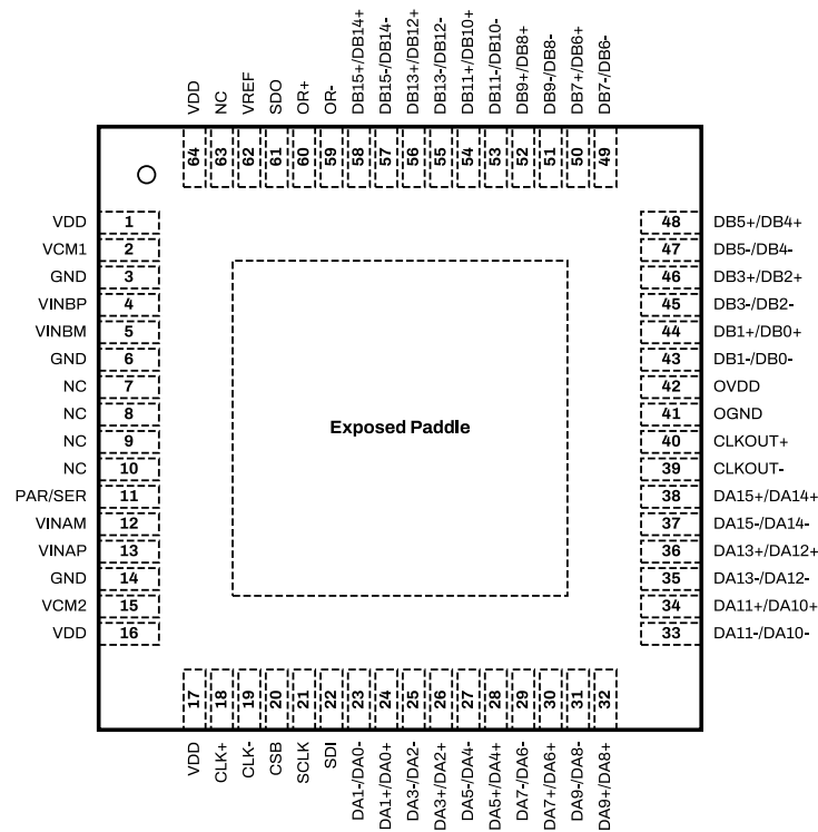
Figure 7: SD2180 Package Top View for Channel Multiplexed LVDS Configuration.
