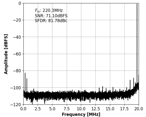
Figure 11: Single-Tone FFT with f_{IN}=220\text{MHz} .
