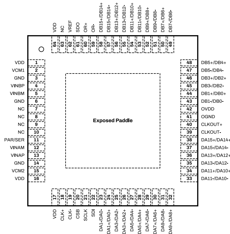
Figure 7: SD2182 Package Top View for Channel Multiplexed LVDS Configuration.
