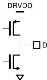
Figure 23: Equivalent Digital Output Circuit.
