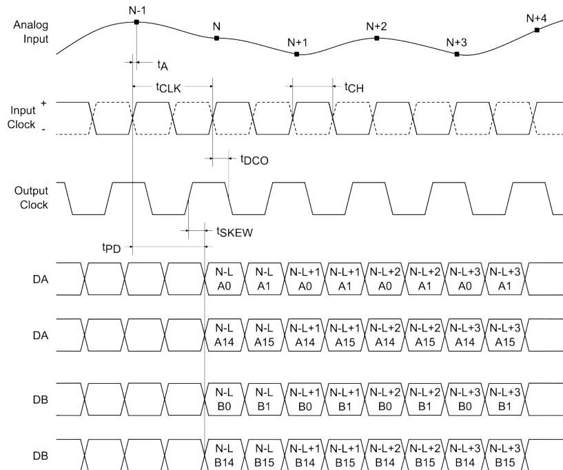
Figure 4: Channel Multiplexed LVDS Output Mode Timing.
