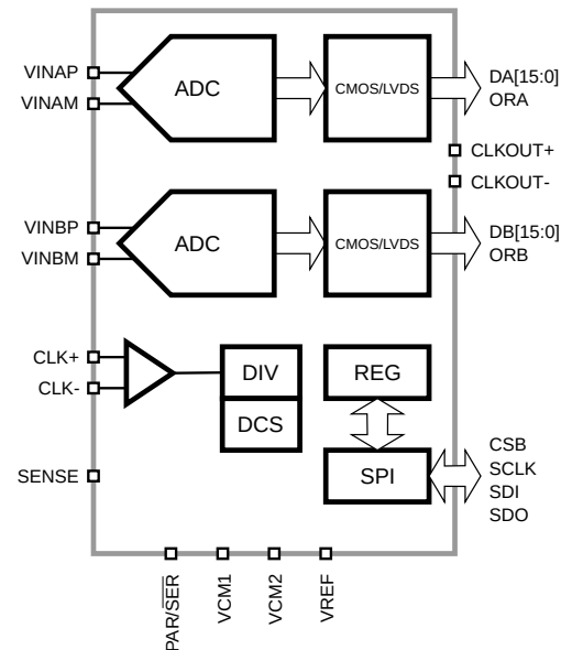
Figure 1: SD2182 Functional Block Diagram.
