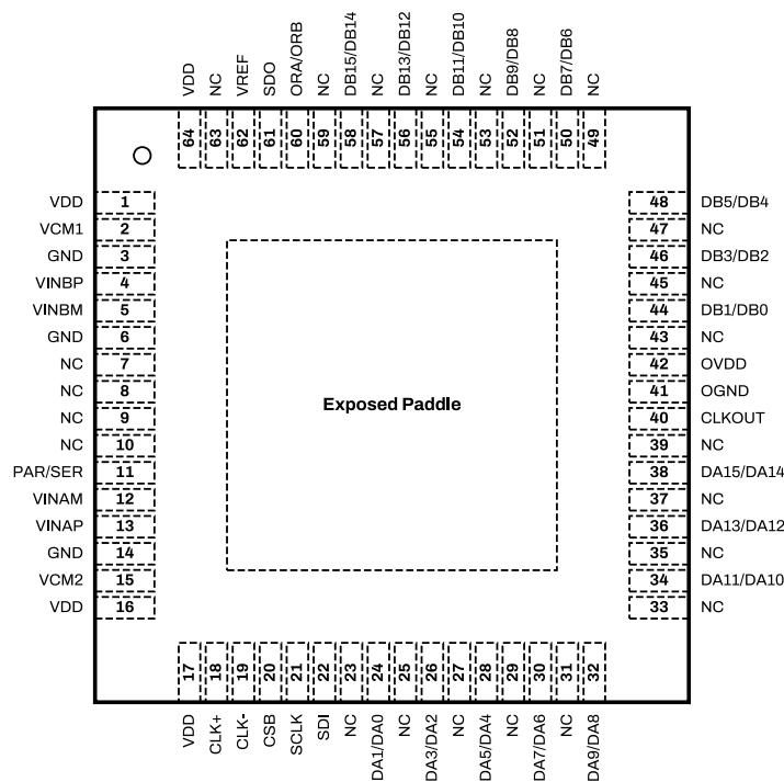
Figure 6: SD2182 Package Top View for Channel Multiplexed CMOS Configuration.
