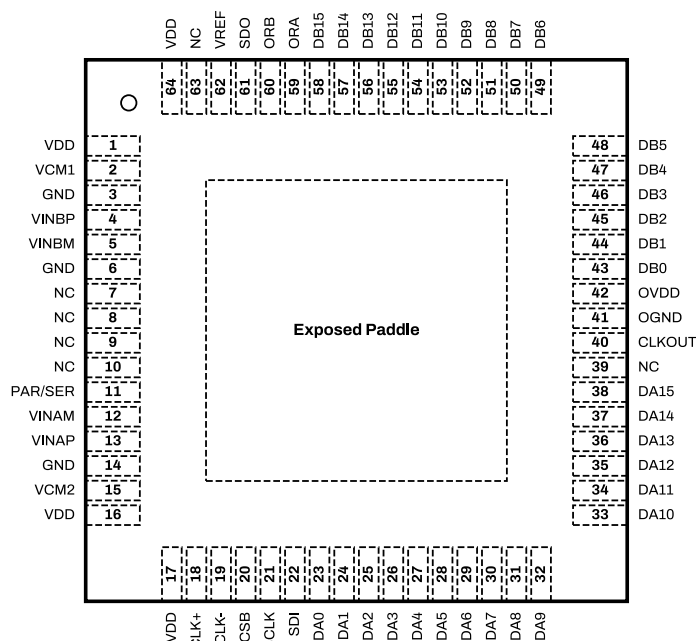
Figure 5: SD2183 Package Top View for Parallel CMOS Configuration.
