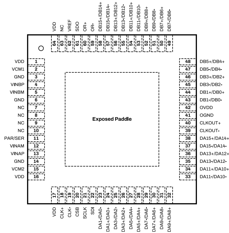
Figure 7: SD2183 Package Top View for Channel Multiplexed LVDS Configuration.
