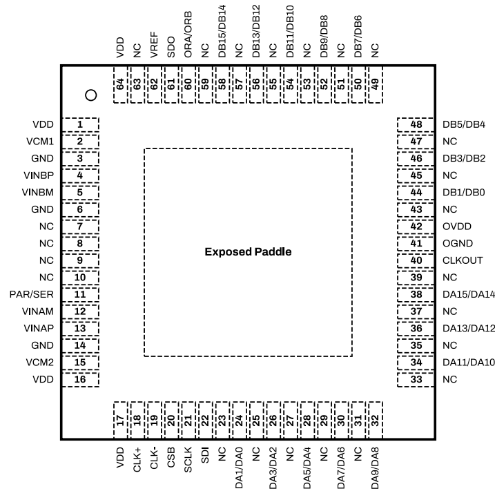
Figure 6: SD2183 Package Top View for Channel Multiplexed CMOS Configuration.
