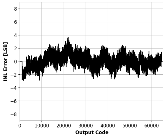
Figure 14: INL Error with f_{IN}=6.55\text{MHz} .
