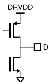
Figure 23: Equivalent Digital Output Circuit.
