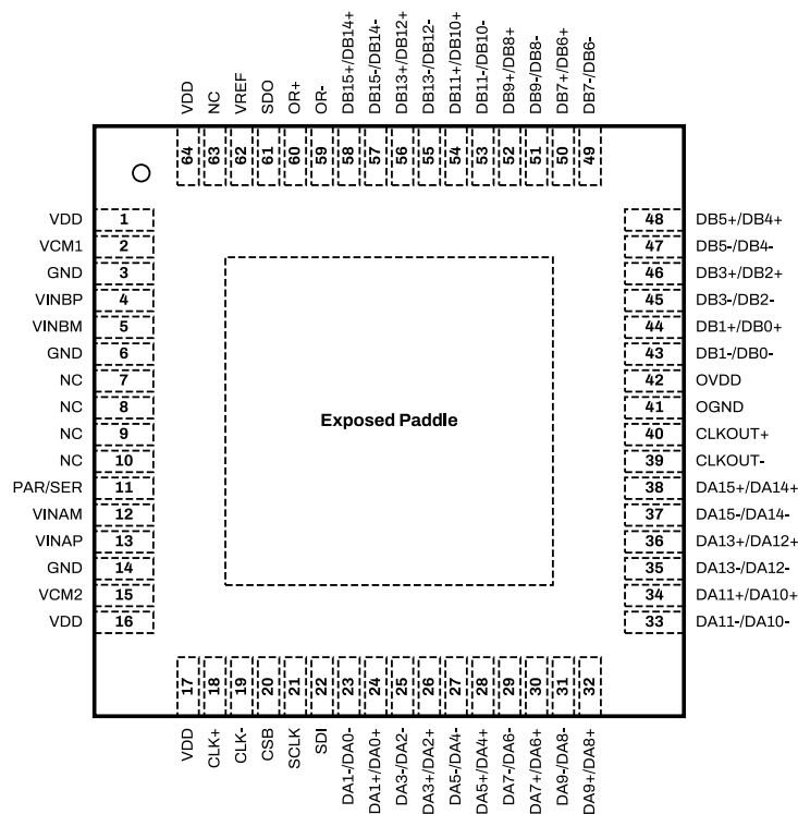
Figure 7: SD2185 Package Top View for Channel Multiplexed LVDS Configuration.
