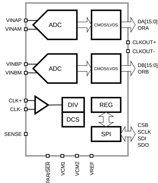
Figure 1: SD2185 Functional Block Diagram.
