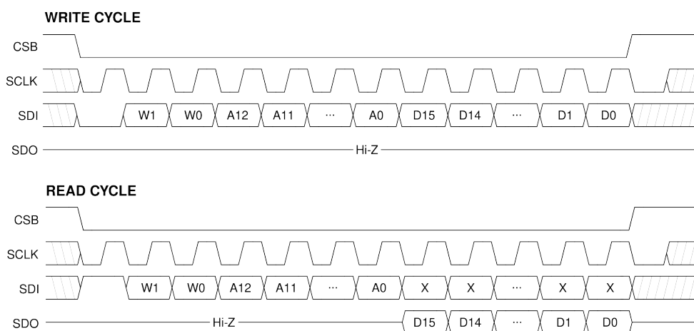
Figure 25: 4-wire SPI timing.
