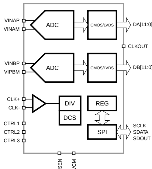
Figure 1: SD4222 Functional Block Diagram.
