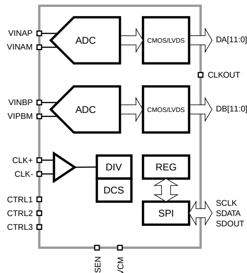
Figure 1: SD4229 Functional Block Diagram.
