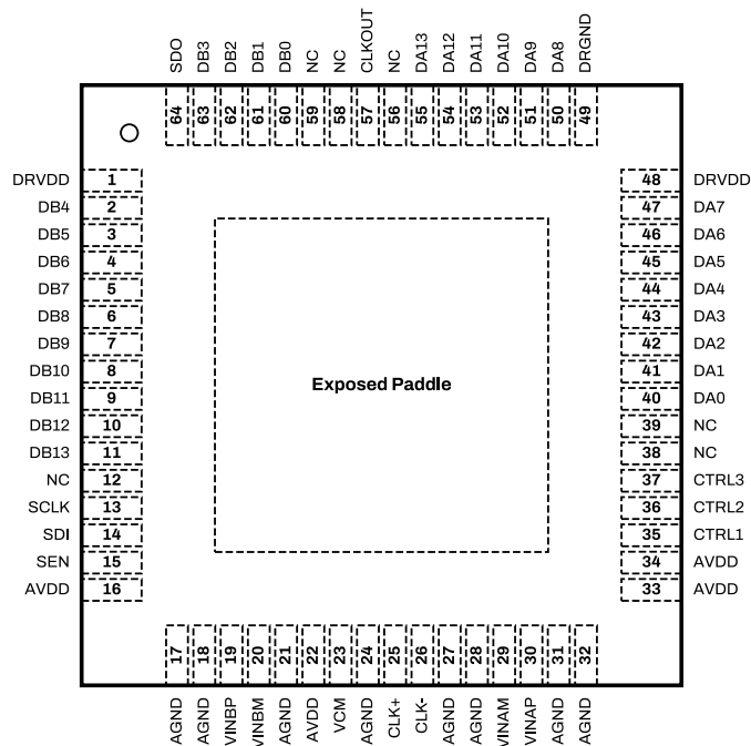
Figure 4: SD4242 Package Top View for Parallel CMOS Configuration.
