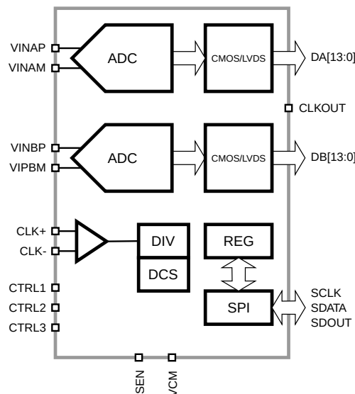
Figure 1: SD4242 Functional Block Diagram.
