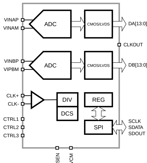
Figure 1: SD4245 Functional Block Diagram.
