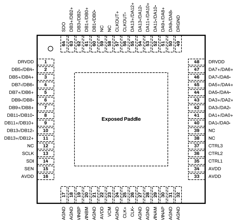
Figure 5: SD4245 Package Top View for Channel Multiplexed LVDS Configuration.
