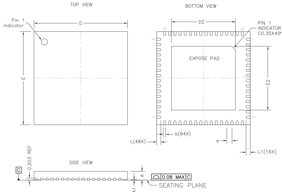
Figure 26: Package Dimensions.
