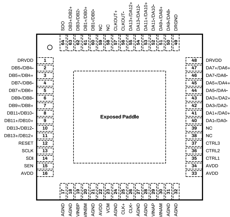
Figure 5: SD4246 Package Top View for Channel Multiplexed LVDS Configuration.
