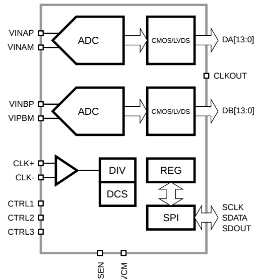
Figure 1: SD4246 Functional Block Diagram.
