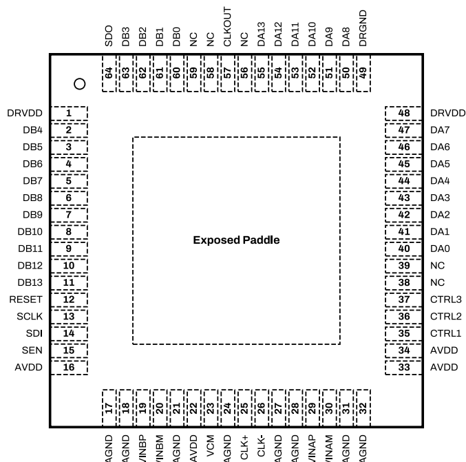
Figure 4: SD4246 Package Top View for Parallel CMOS Configuration.
