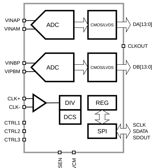
Figure 1: SD4249 Functional Block Diagram.
