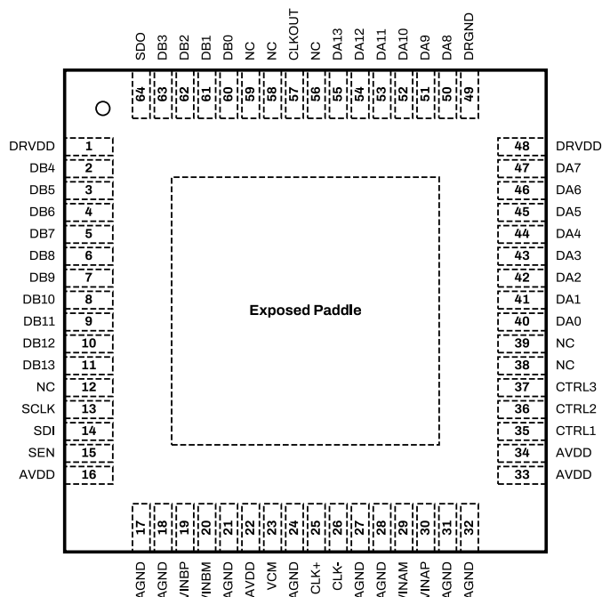
Figure 4: SD4249 Package Top View for Parallel CMOS Configuration.
