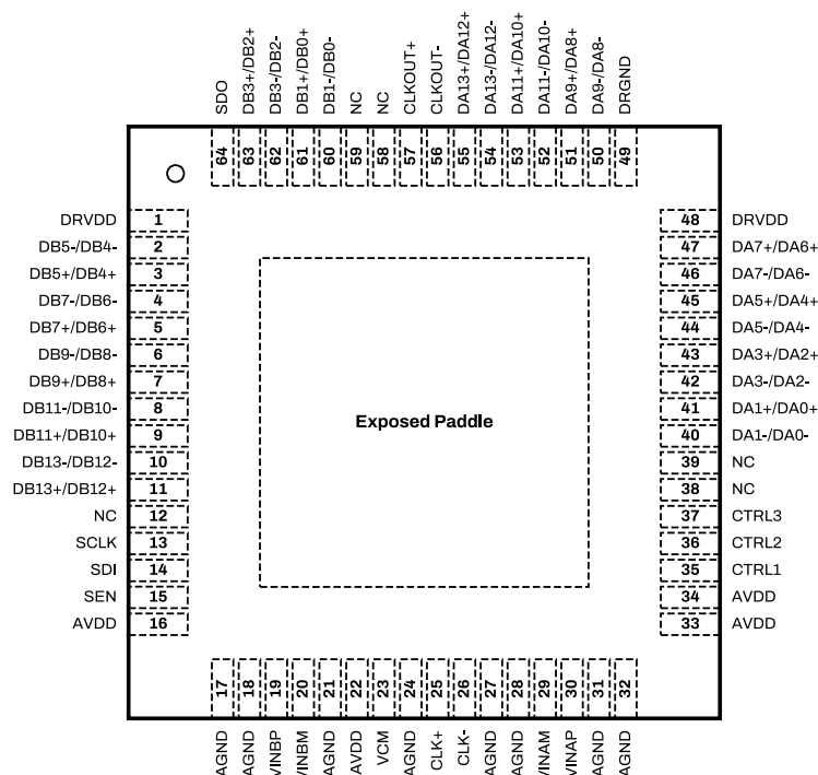
Figure 5: SD4249 Package Top View for Channel Multiplexed LVDS Configuration.
