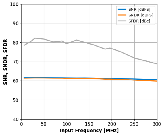
Figure 15: Single-Tone SNR, SNDR and SFDR vs. Input Frequency with f_S=20\text{MHz} .
