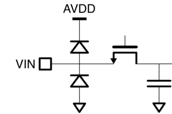
Figure 19: Equivalent Analog Input Circuit.
