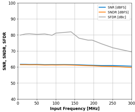
Figure 15: Single-Tone SNR, SNDR and SFDR vs. Input Frequency with f_S=40\text{MHz} .
