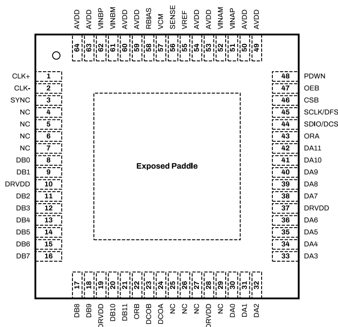
Figure 5: SD9231 Package Top View for Parallel CMOS Configuration.
