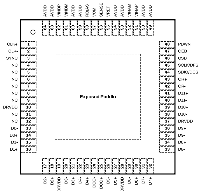
Figure 6: SD9231 Package Top View for Parallel LVDS Configuration.
