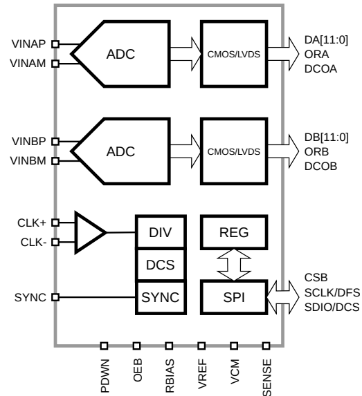
Figure 1: SD9231 Functional Block Diagram.
