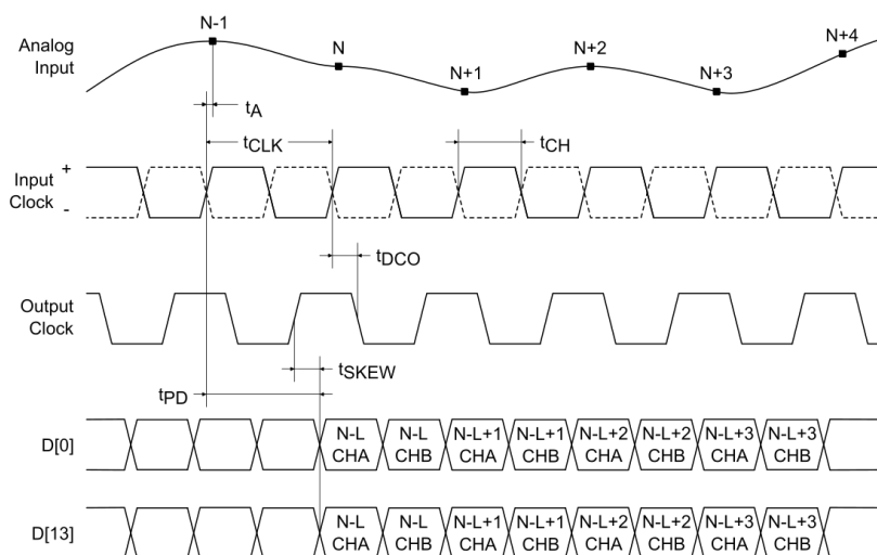
Figure 4: Parallel LVDS Output Mode Timing.
