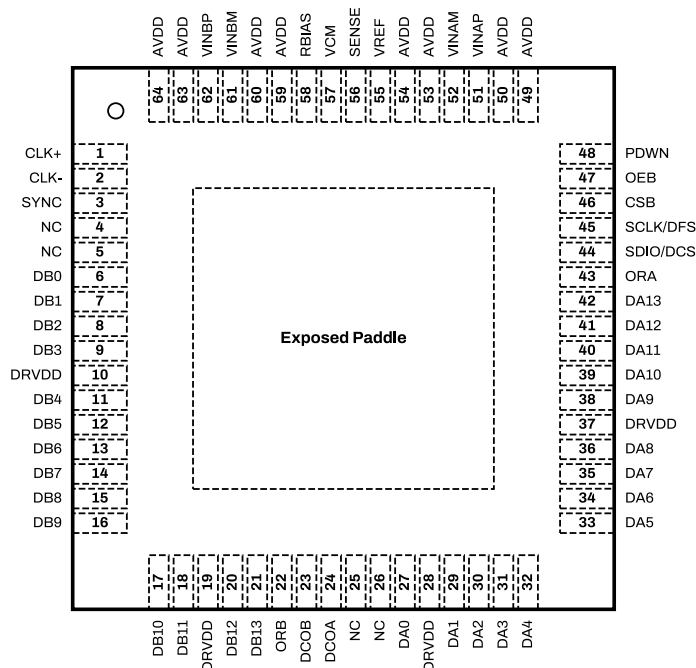
Figure 5: SD9251 Package Top View for Parallel CMOS Configuration.
