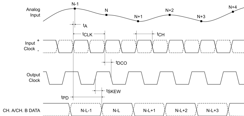
Figure 3: Parallel CMOS Output Mode Timing.
