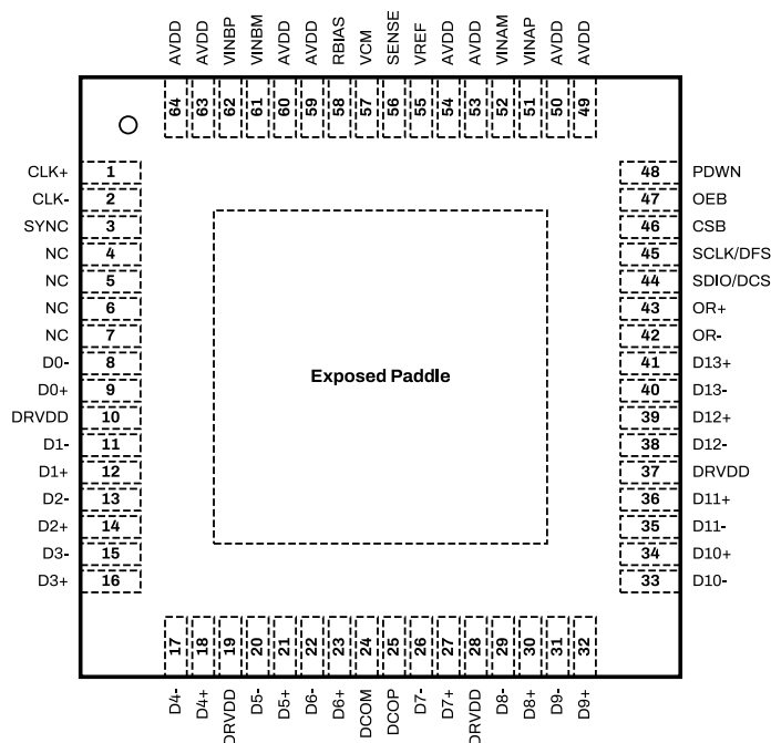
Figure 6: SD9251 Package Top View for Parallel LVDS Configuration.
