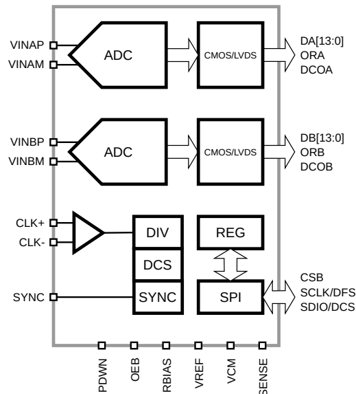
Figure 1: SD9258 Functional Block Diagram.
