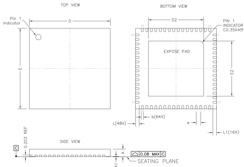
Figure 31: Package Dimensions.
