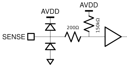
Figure 30: Equivalent SENSE Input Circuit.
