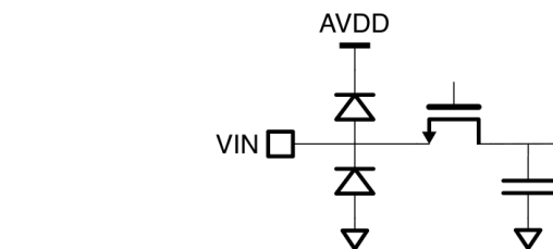
Figure 21: Equivalent Analog Input Circuit.
