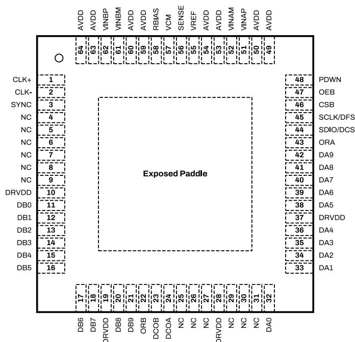
Figure 6: SD9608 Package Top View for Parallel CMOS Configuration.
