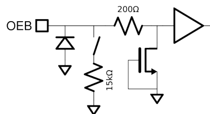
Figure 25: Equivalent OEB Input Circuit.
