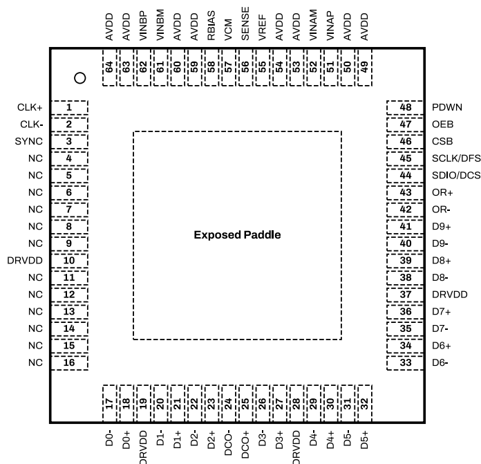
Figure 7: SD9608 Package Top View for Parallel LVDS Configuration.
