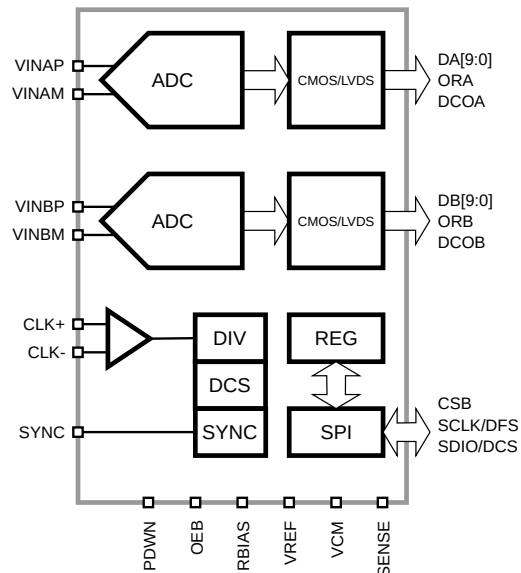
Figure 1: SD9608 Functional Block Diagram.
