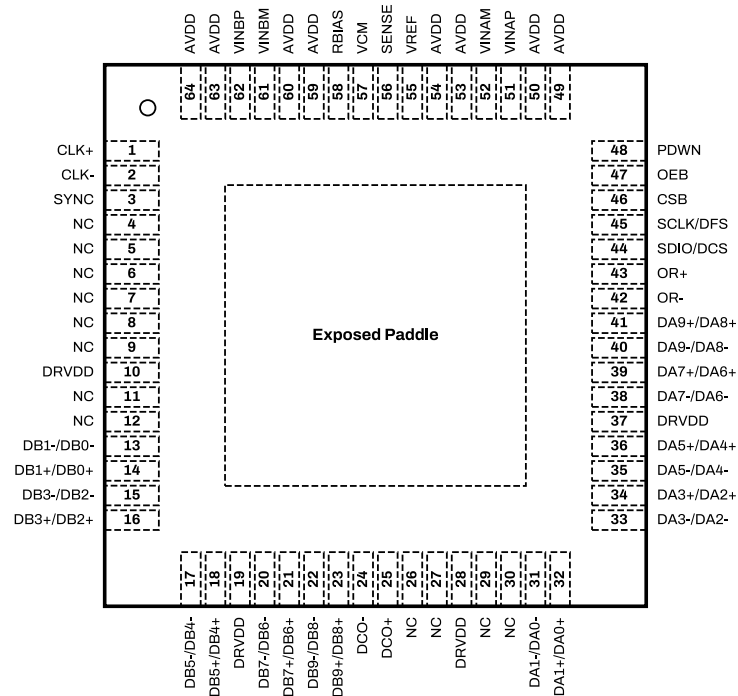
Figure 8: SD9608 Package Top View for Channel Multiplexed LVDS Configuration.
