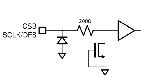
Figure 24: Equivalent CSB or SCLK/DFS Input Circuit.
