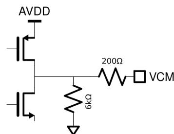
Figure 23: Equivalent VCM Circuit.
