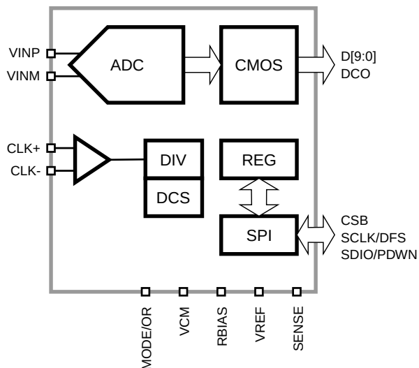
Figure 1: SD9609 Functional Block Diagram.
