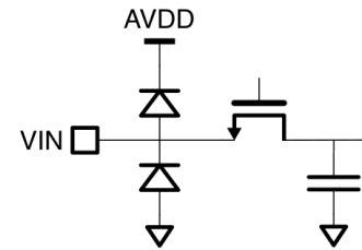
Figure 16: Equivalent Analog Input Circuit.
