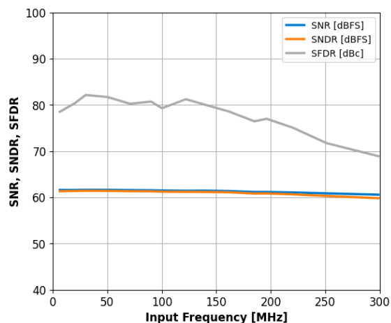
Figure 12: Single-Tone SNR, SNDR and SFDR vs. Input Frequency with f_S=20\text{MHz} .
