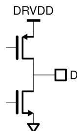
Figure 20: Equivalent Digital Output Circuit.
