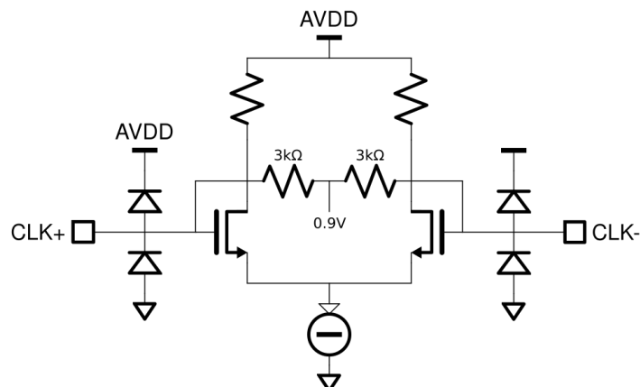
Figure 15: Equivalent Clock Input Circuit.
