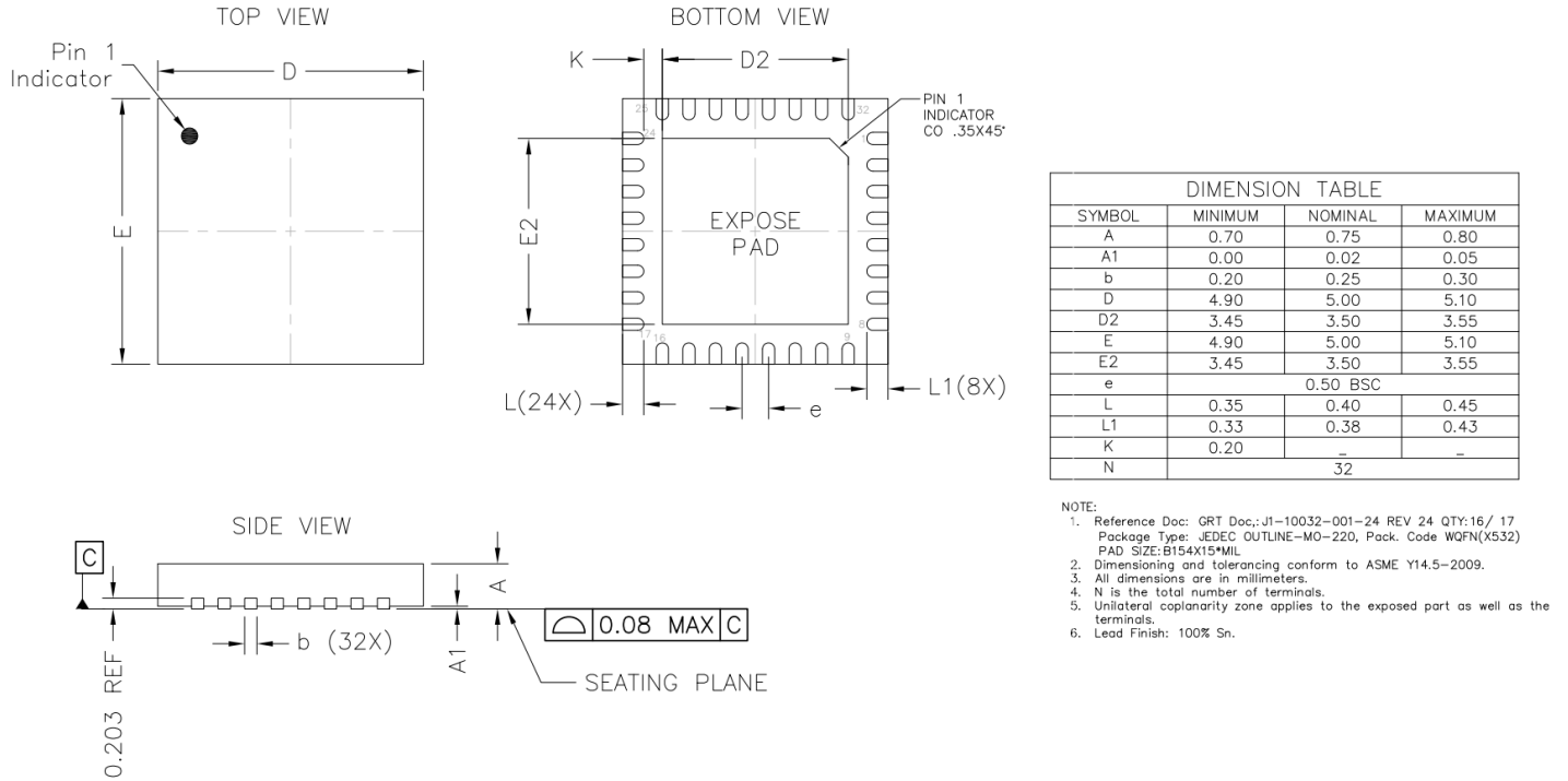
Figure 24: Package Dimensions.
