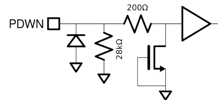
Figure 24: Equivalent PDWN Input Circuit.
