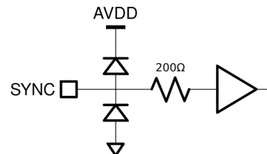
Figure 26: Equivalent SYNC Input Circuit.
