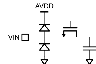
Figure 22: Equivalent Analog Input Circuit.
