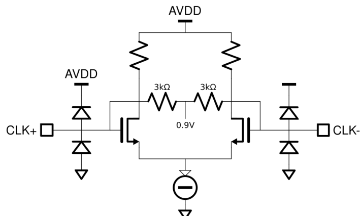
Figure 21: Equivalent Clock Input Circuit.
