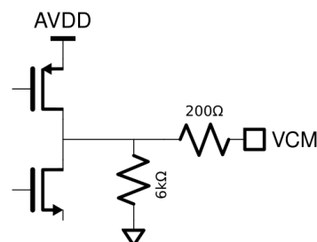
Figure 24: Equivalent VCM Circuit.
