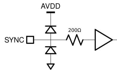
Figure 30: Equivalent SYNC Input Circuit.
