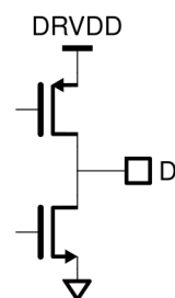
Figure 28: Equivalent Digital Output Circuit.
