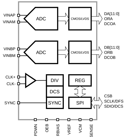
Figure 1: SD9628 Functional Block Diagram.
