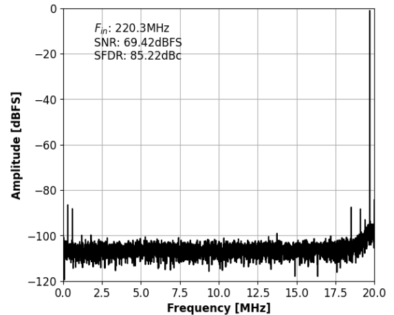
Figure 7: Single-Tone FFT with f_{IN}=220\text{MHz} .
