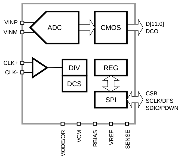
Figure 1: SD9629 Functional Block Diagram.
