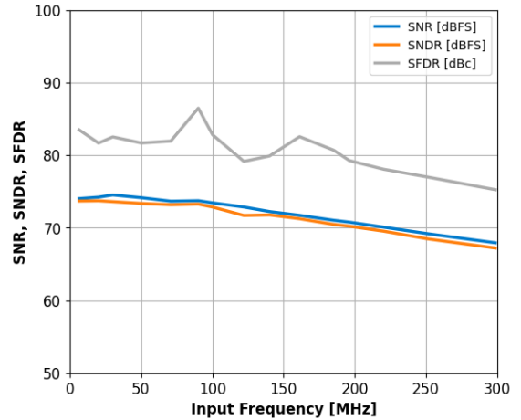
Figure 14: Single-Tone SNR, SNDR and SFDR vs. Input Frequency with f_S=210\text{MHz} .
