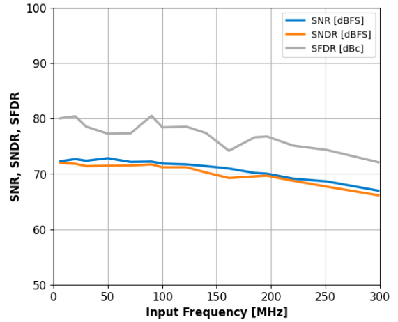
Figure 14: Single-Tone SNR, SNDR and SFDR vs. Input Frequency with f_S=250\text{MHz} .
