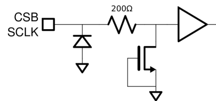
Figure 20: Equivalent CSB or SCLK Input Circuit.
