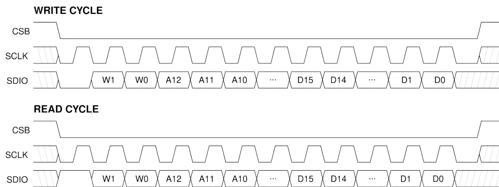
Figure 25: 3-wire SPI timing.
