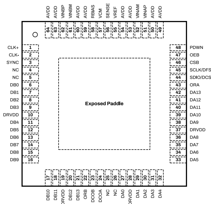
Figure 5: SD9648 Package Top View for Parallel CMOS Configuration.
