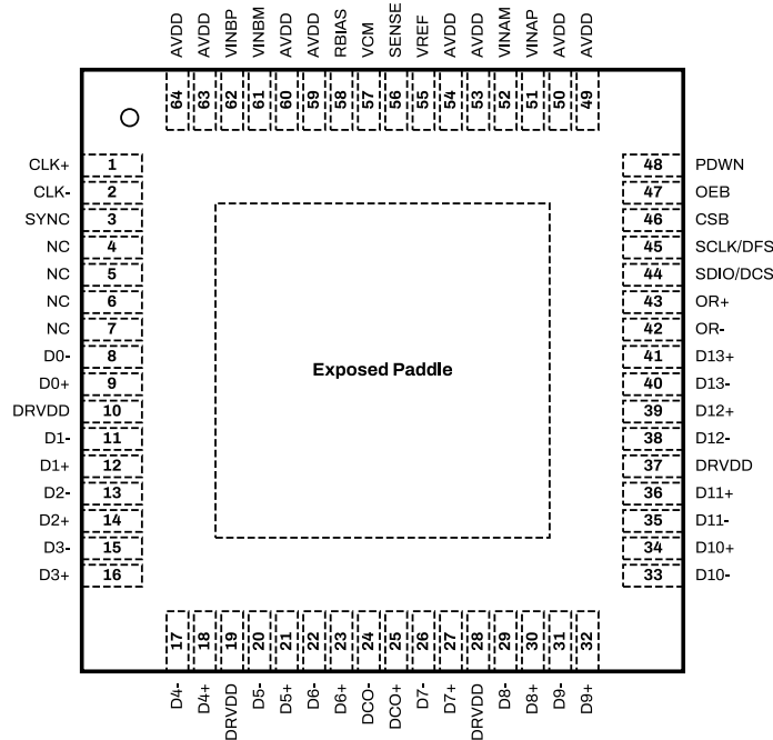
Figure 6: SD9648 Package Top View for Interleaved Parallel LVDS Configuration.
