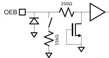
Figure 24: Equivalent OEB Input Circuit.
