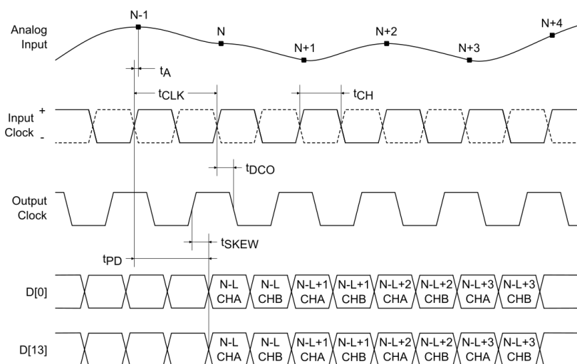
Figure 4: Interleaved Parallel LVDS Output Mode Timing.
