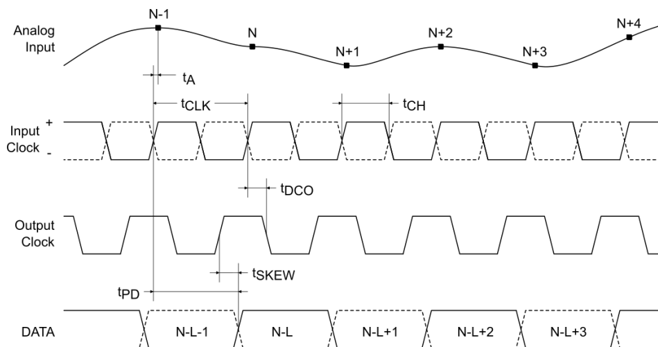
Figure 2: Parallel CMOS Output Mode Timing.
