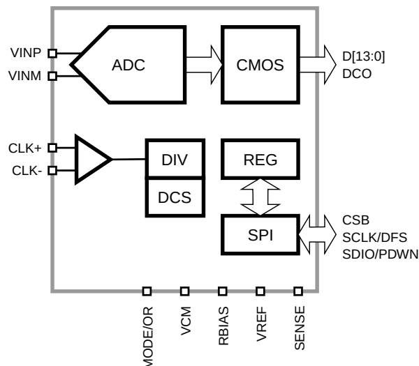
Figure 1: SD9649 Functional Block Diagram.
