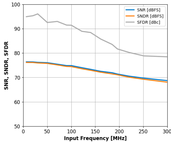
Figure 15: Single-Tone SNR, SNDR and SFDR vs. Input Frequency with f_S=25\text{MHz} .
